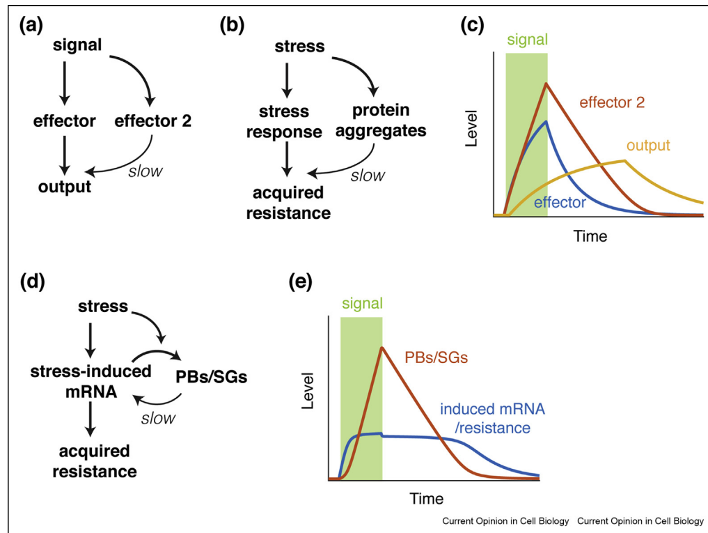
Feedforward loops allow the spreading of signal effects in time. (a) Topology of a general feedforward loop. (b) An example of a feedforward loop that generates cellular memory through signal-induced protein aggregation. (c) The time trace of a feedforward system that enables a long-lasting response to a transient signal. Green, signal; blue, effector; red, effector 2 (slow); yellow, output. (d) An example of a variant of feedforward loops that generates cellular memory through signal-induced mRNA storage in PBs/SGs. (e) The time trace of the feedback forward system in (d) that enables long-lasting plateau of gene expression response and acquired stress resistance upon a transient stimulus. Green signal; red, mRNAs stored in PBs/SGs; blue, stress-induced functional mRNAs/acquired stress resistance. PBs, processing bodies; SGs, stress granules.
